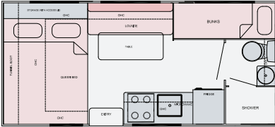
16'6ft Single Axle Model
