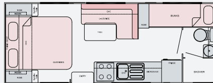
19'6ft Tandem Axle Model
