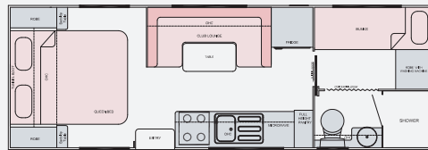
22ft Tandem Axle Model
