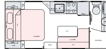
16'6ft Single Axle Model
